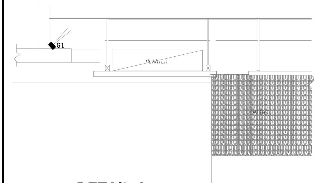
DETAIL A G1 GAMING CEILING STRIP LIGHT SECTION SCALE 1:10
