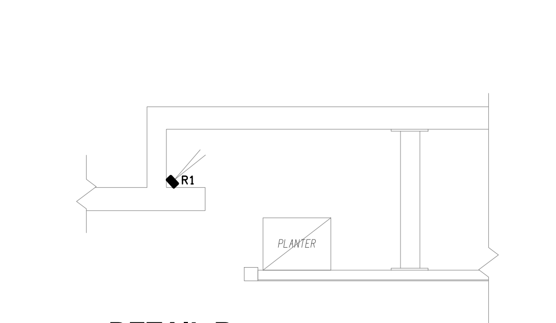
DETAIL B R1 GAMING RECTANGULAR STRIP LIGHT SECTION SCALE 1:10
